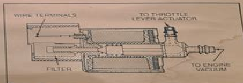
Figure 7-5. Throttle Return Control Solenoid Vacuum Control Valve
