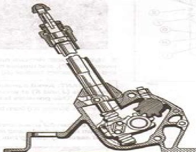
FIG. 1 SECTIONAL VIEW OF STEERING BOX
