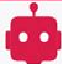
Artificial Intelligence
