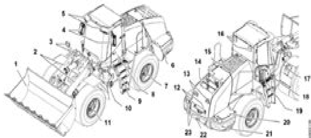
1 Bucket 9 Gate access 17 Wheel wedge 2 Lift arms 10 Articulation lock 18 Fuel tank 3 Front lights 11 Front axle 19 Emergency exit steps 4 Exterior mirror 12 License plate lights (optional) 20 Battery compartment cover 5 Front working headlights 13 Rear working headlights 21 Right ballast weight 6 Left ballast weight 14 Engine compartment hood 22 Towing device 7 Rear axle 15 Cooling system grille 23 Rear lighting 8 Driver's cab 16 Rear working headlight (optional)
