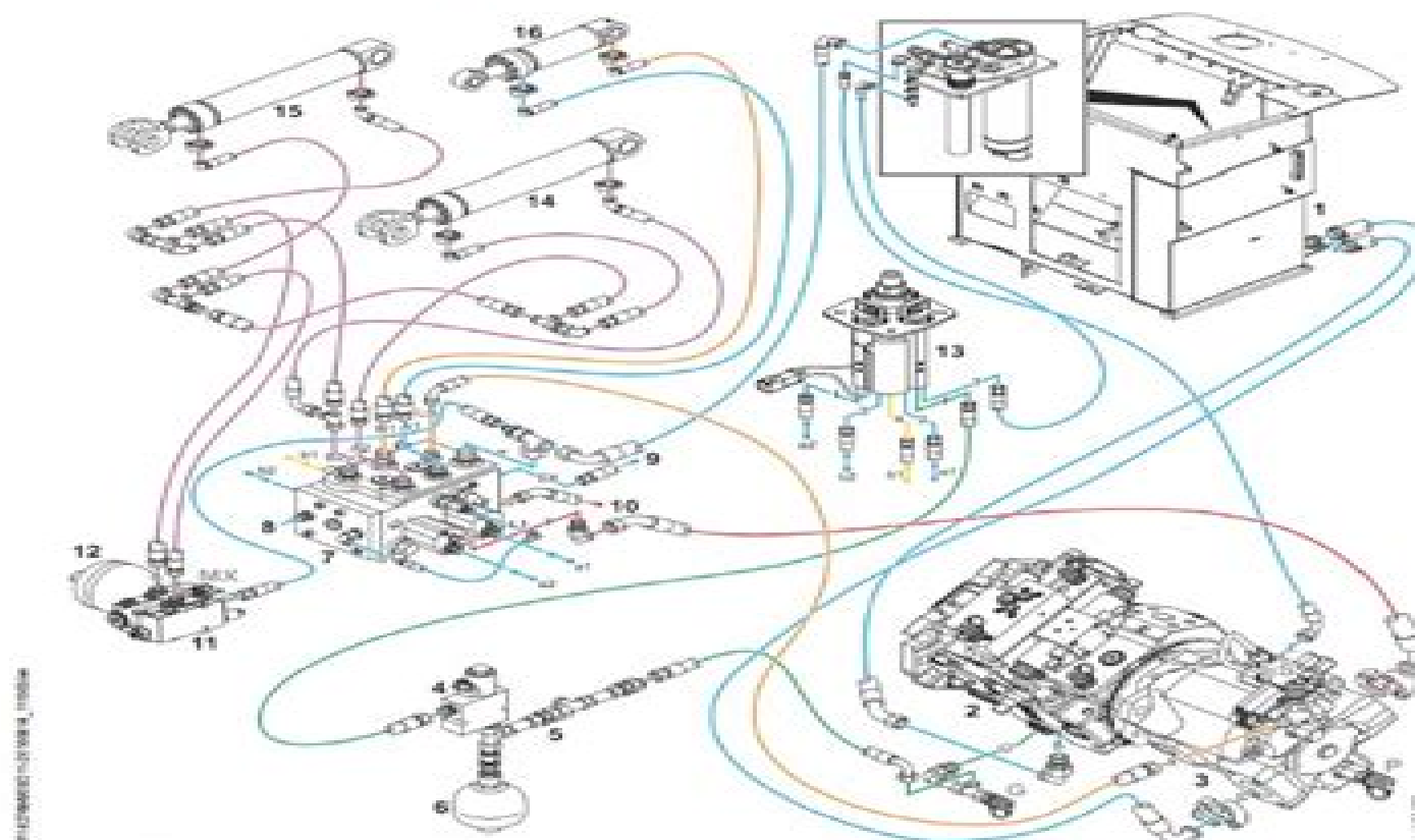
Fig. 232: Main components of the working hydraulics for z-bar kinematics
