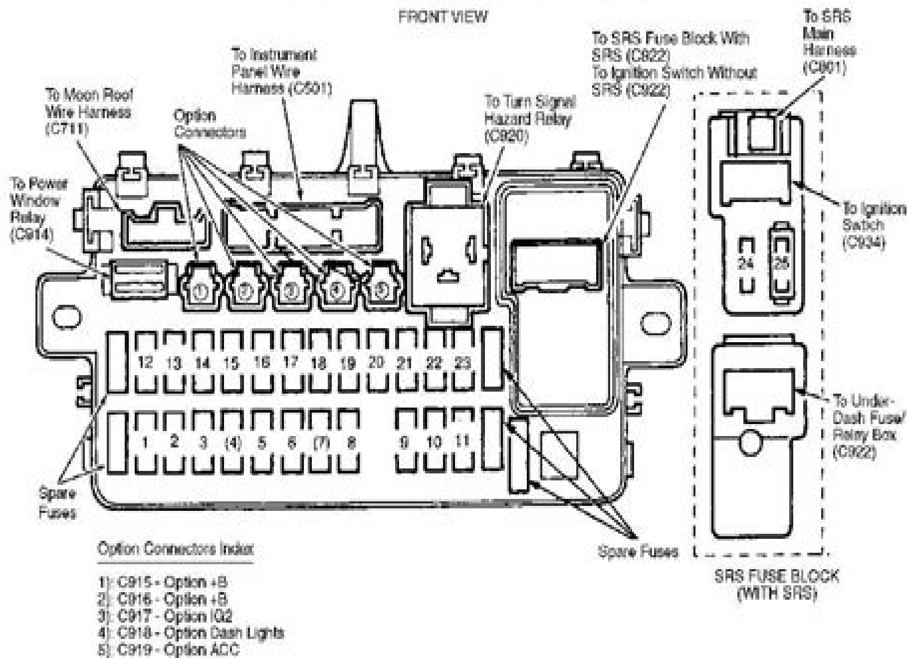
Fig. 5: Identifying Under-Dash Fuse/Relay Box Components (1994-95 Civic)
