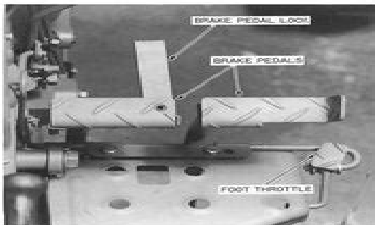
Figure 8 — Foot Throttle and Brake Controls
