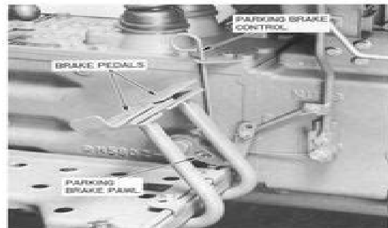
Figure 9 — Parking Brake Control
