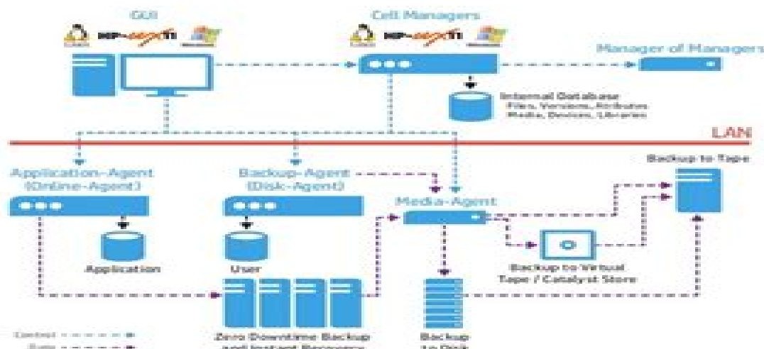
HP Data Protector architecture
