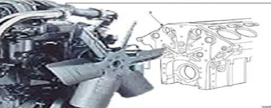
Figure 1-8 Attach a suitable lifting bracket to the end of the front cylinder block, with two 1/2 in. x 10
