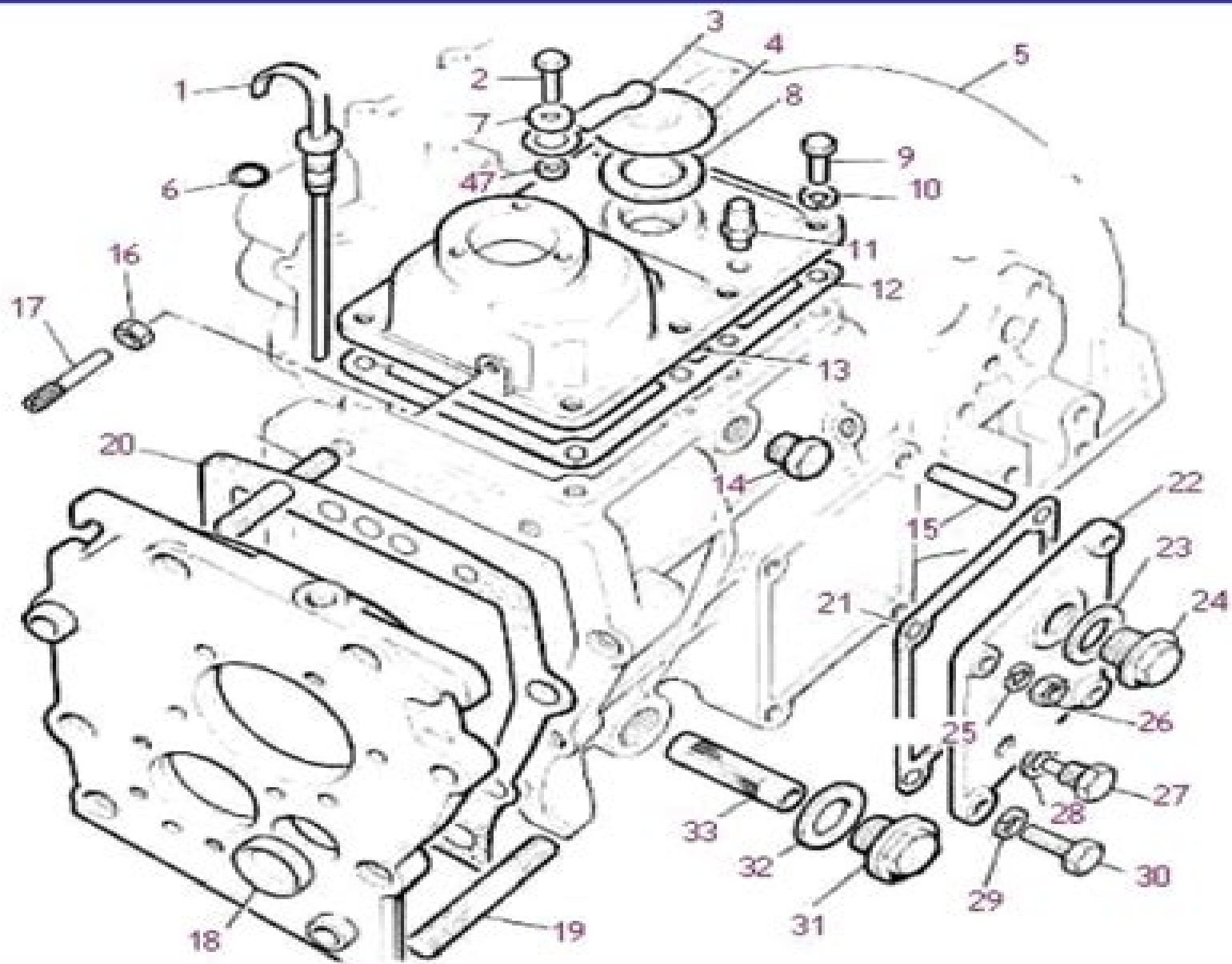
Gearbox
