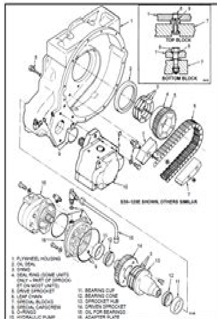
FIGURE 1. PARTS OF CRANK DRIVE ASSEMBLY
