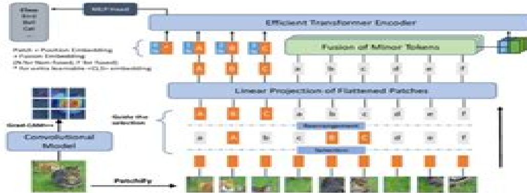
Figure 1: The overview of activation guided attention in our model. After partitioning the input image into patches of fixed size, the heat map produced by Grad-CAM++ via the auxiliary convolutional model M_{conv} is utilized to choose the major tokens and the minor tokens. Then, for each patch, we perform a linear embedding. The minor tokens (grey tokens) are combined into several representation tokens ( N_f < N_m ) via a fusion network in order to decrease computation while preserving background knowledge. After incorporating positional embedding and fusion embedding into tokens, the output is fed into an efficient transformer encoder.
