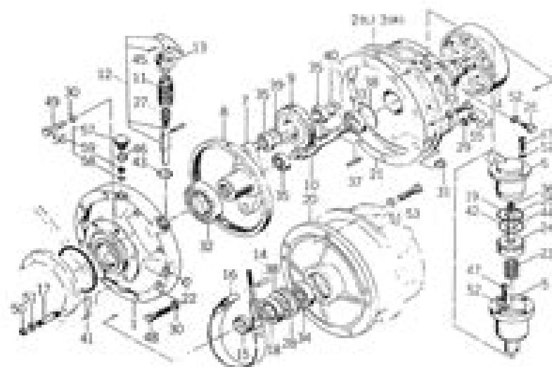
Fig. 4-2-3 Reduction only
