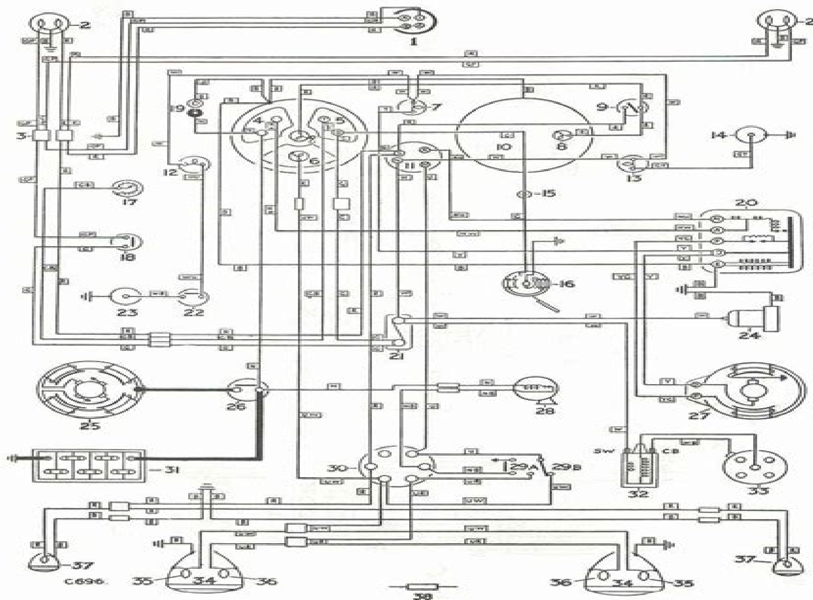
Fig. P-8—Wiring diagram 88 and 109—1954-58 models
