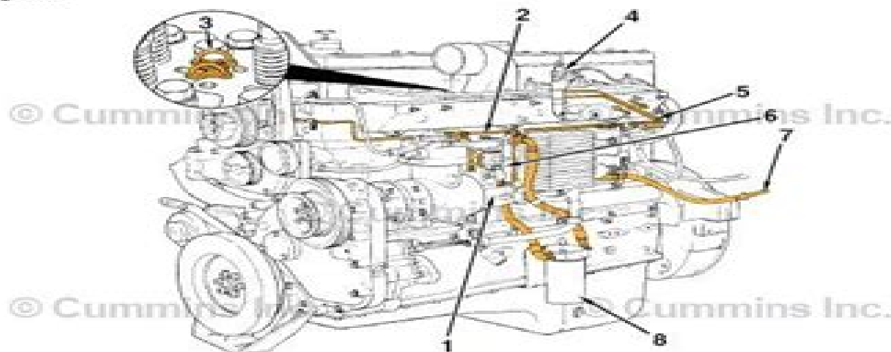
CELECT™ and CELECT™ Plus Fuel System
