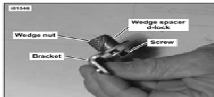
Figure 1. Assemble Left Side Mounting Bracket
