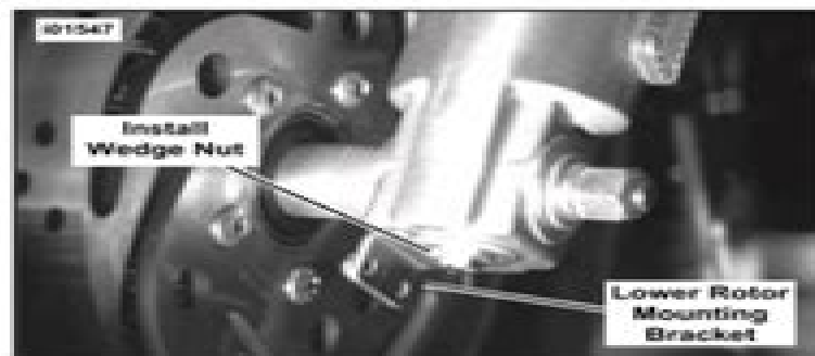
Figure 2. Install Lower Rotor Mounting Bracket
