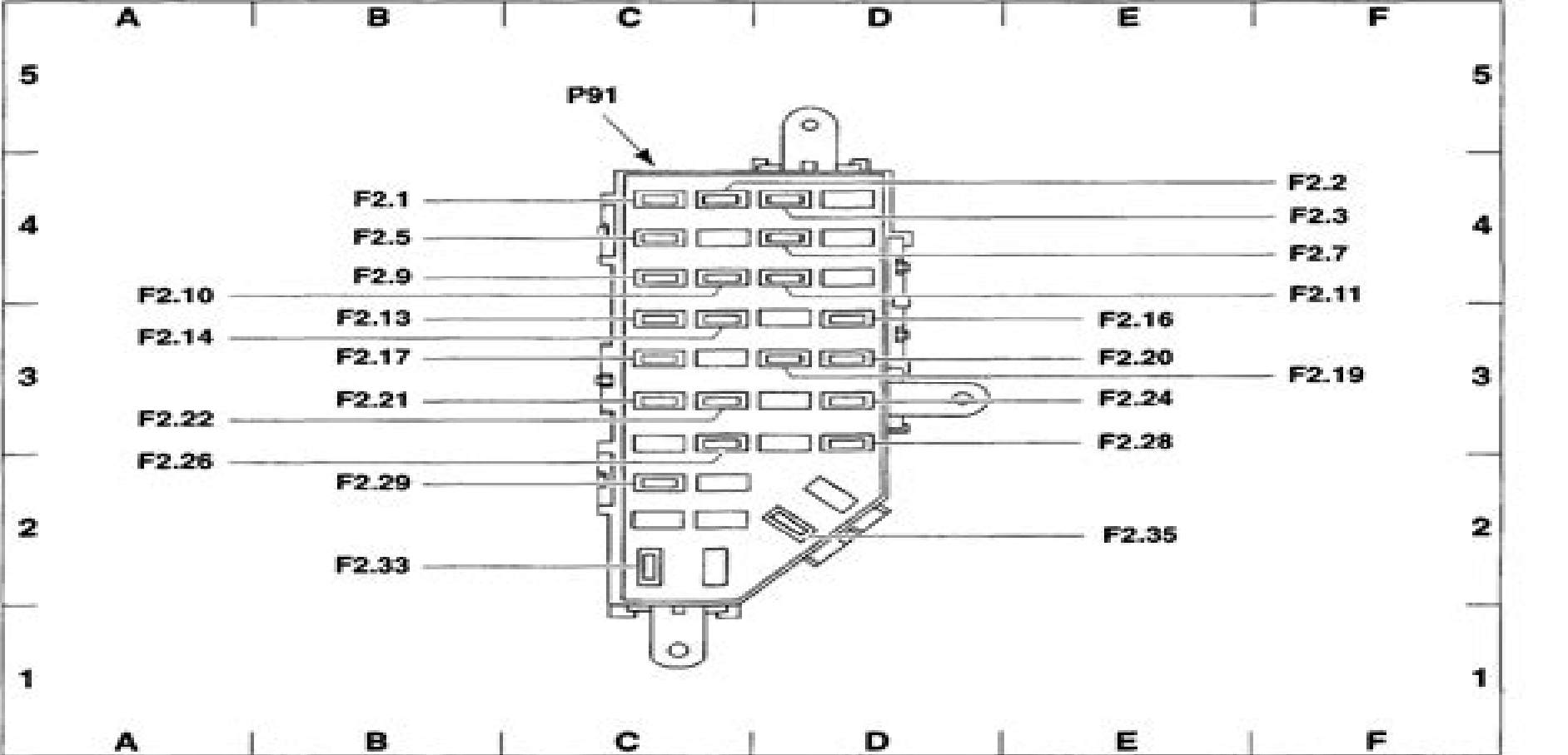
Central Junction Box (CJB)
