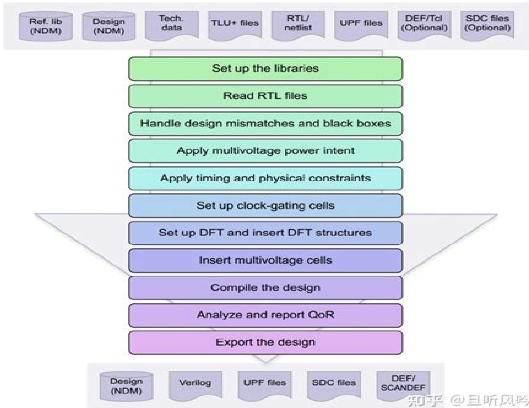
Figure 1 Fusion Compiler Physical Synthesis Flow
