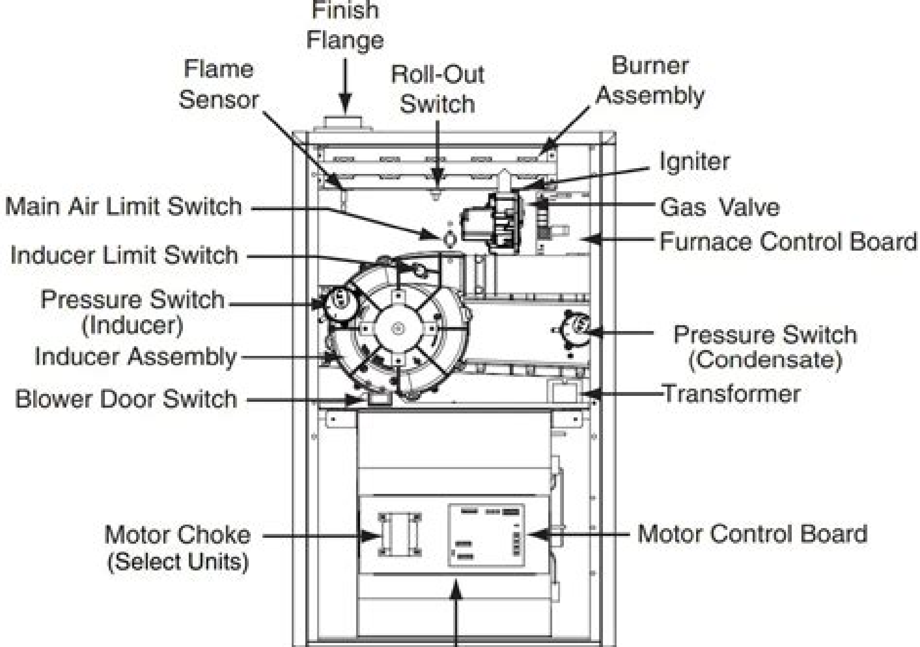
KG7SD Series -Upflow / Horizontal Furnace
