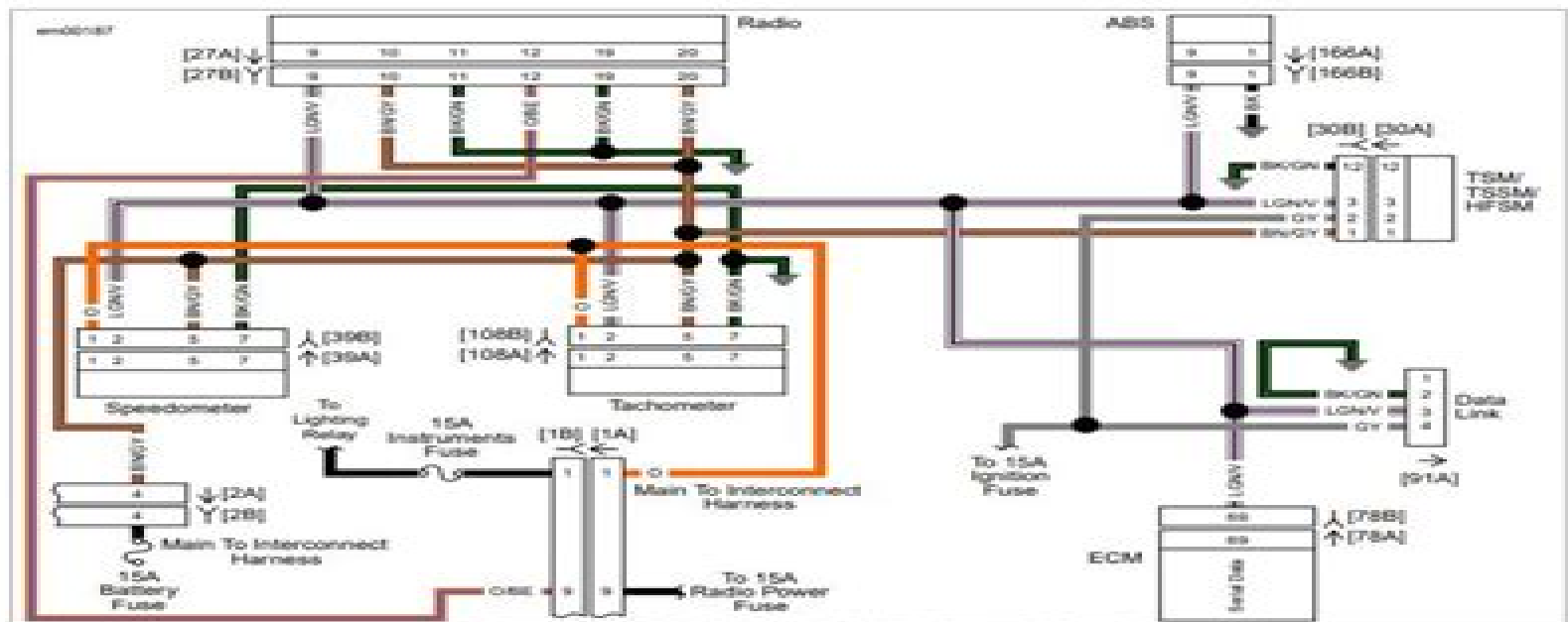
Figure 8-8. J1950 Serial Data Circuit
