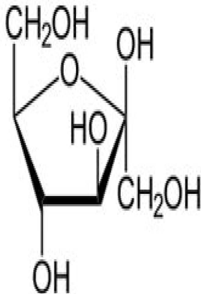
\beta -D-Fructofuranose
