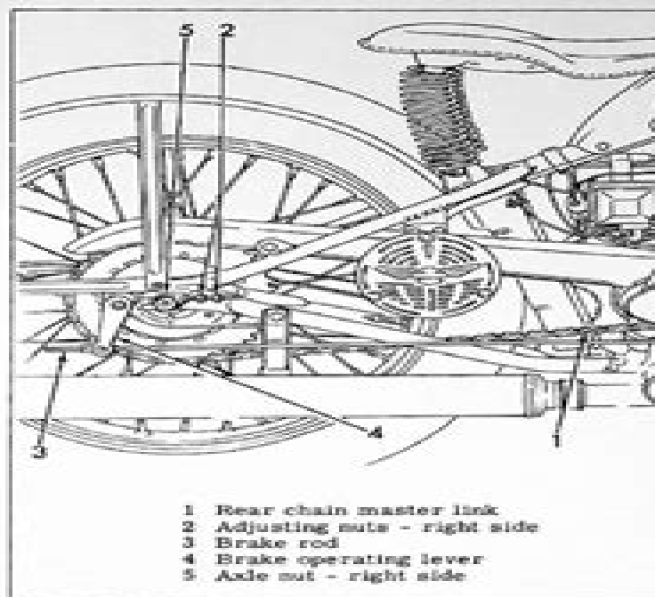
Figure 2C-22. Rear Wheel
