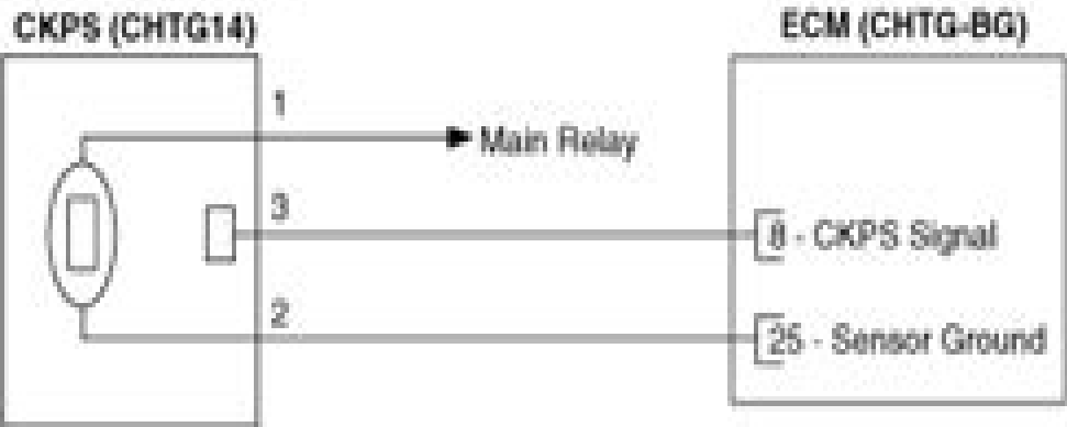
[Harness Connector]
