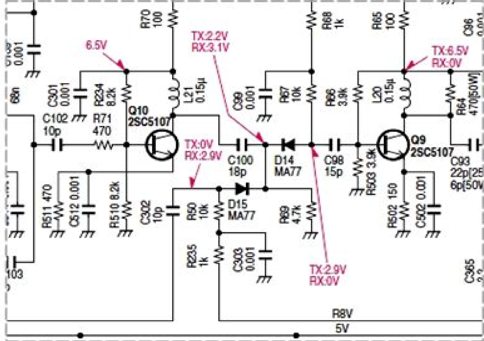
Preview: ICOM IC-F510, F520, F521 schematic diagram
