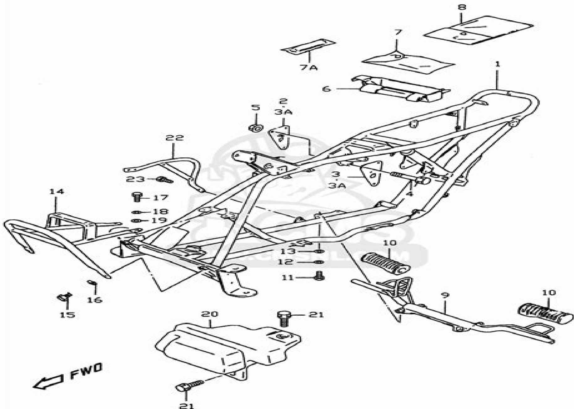
FIG. 14 FRAME - FOOTREST
