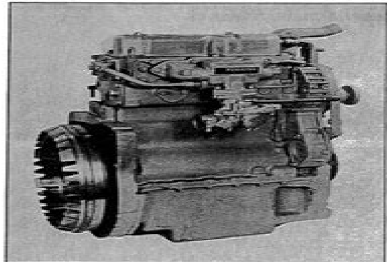
Fig. 2 - Rear Right-Hand View of AG3.152 Engine
