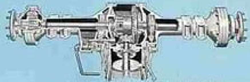
Ruggedly-cased rear axle has final reduction through totally enclosed oil bath epicyclic hub gears giving final drive reduction of 1:10.9. Note also the two implement mounting pads and differential lock foot pedal. Disc brakes acting independently—are sealed against weather, give double-quick turnaround.
