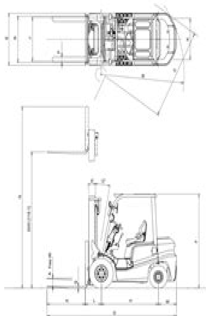
Fig. 1 Track Dimensions
