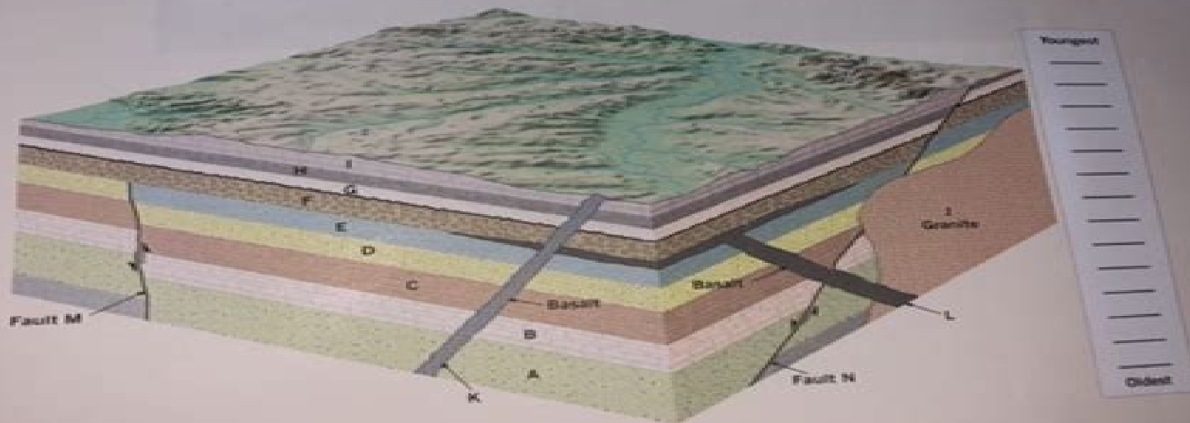
▲ Figure 10.24 Geologic block diagram of a hypothetical region.
