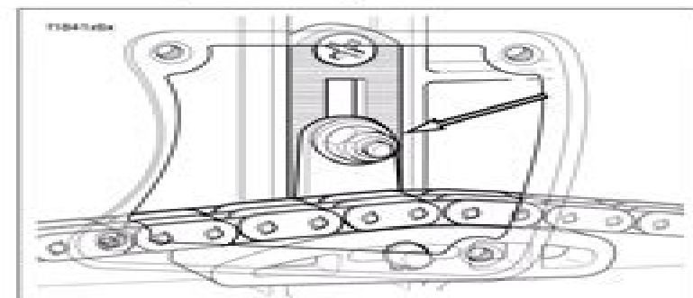
Figure 1-6. Primary Chain Tensioner Assembly
