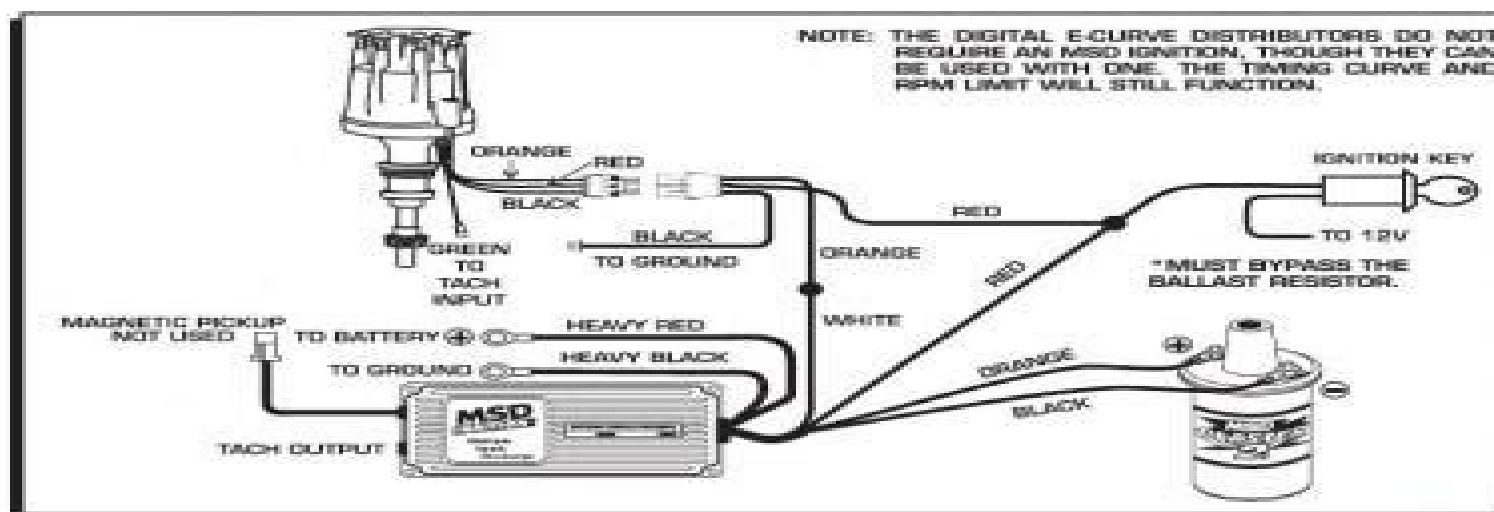
Figure 7 Connecting an MSD Ignition Control to the Digital E-Curve Distributor.
