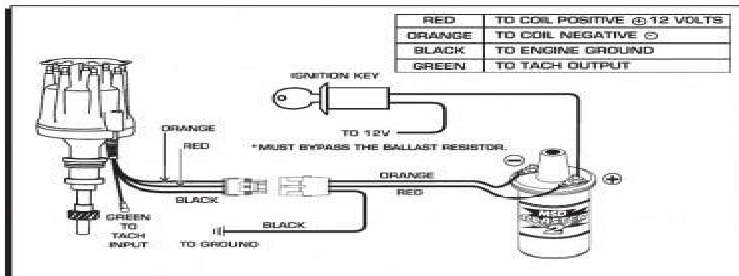
Figure 6 Wiring the Ready-to-Run Chevrolet Distributor.
