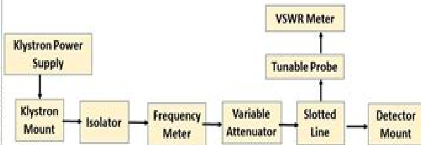
Block diagram of microwave test bench
