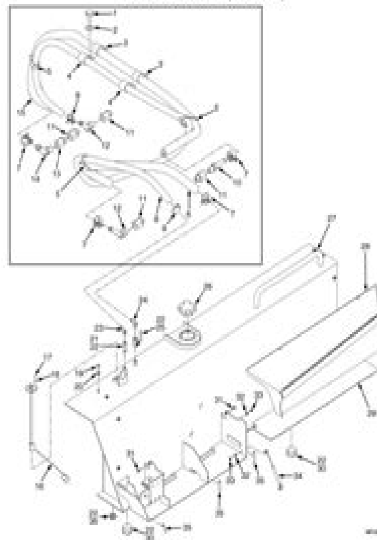
FUEL SUPPLY SYSTEM (FIGURE 3-1)
