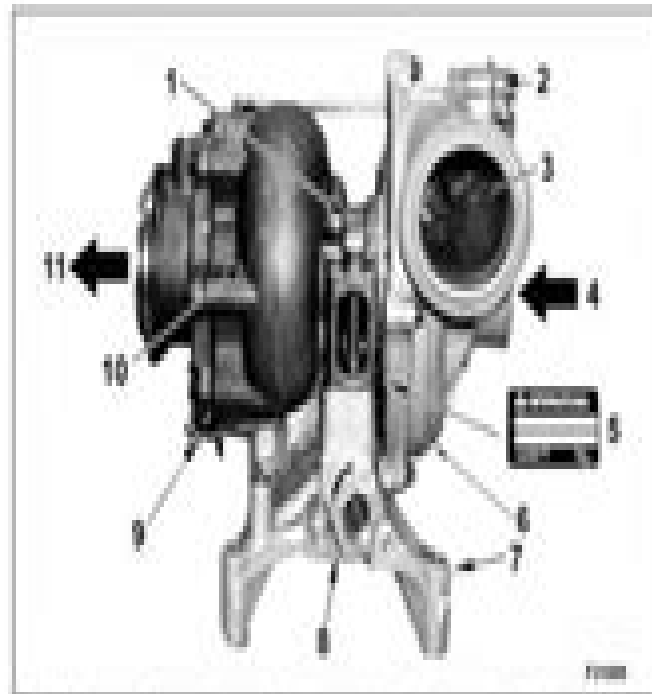
Figure 25 Garrett Turbocharged Turbocharger (L60 200 Through 200 Model Year (1997-00 Model Years))
