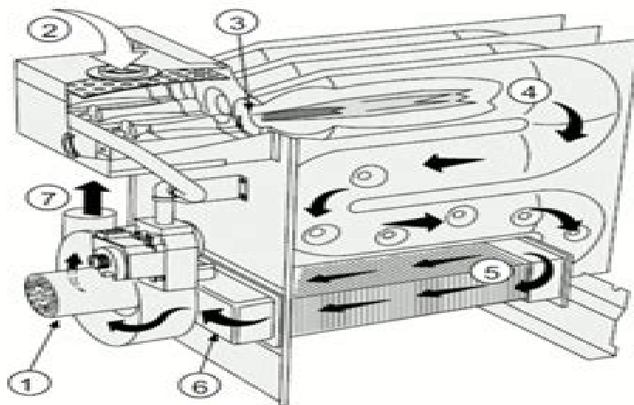
G26 FURNACE ▲ G26 HEAT EXCHANGE ASSEMBLY
