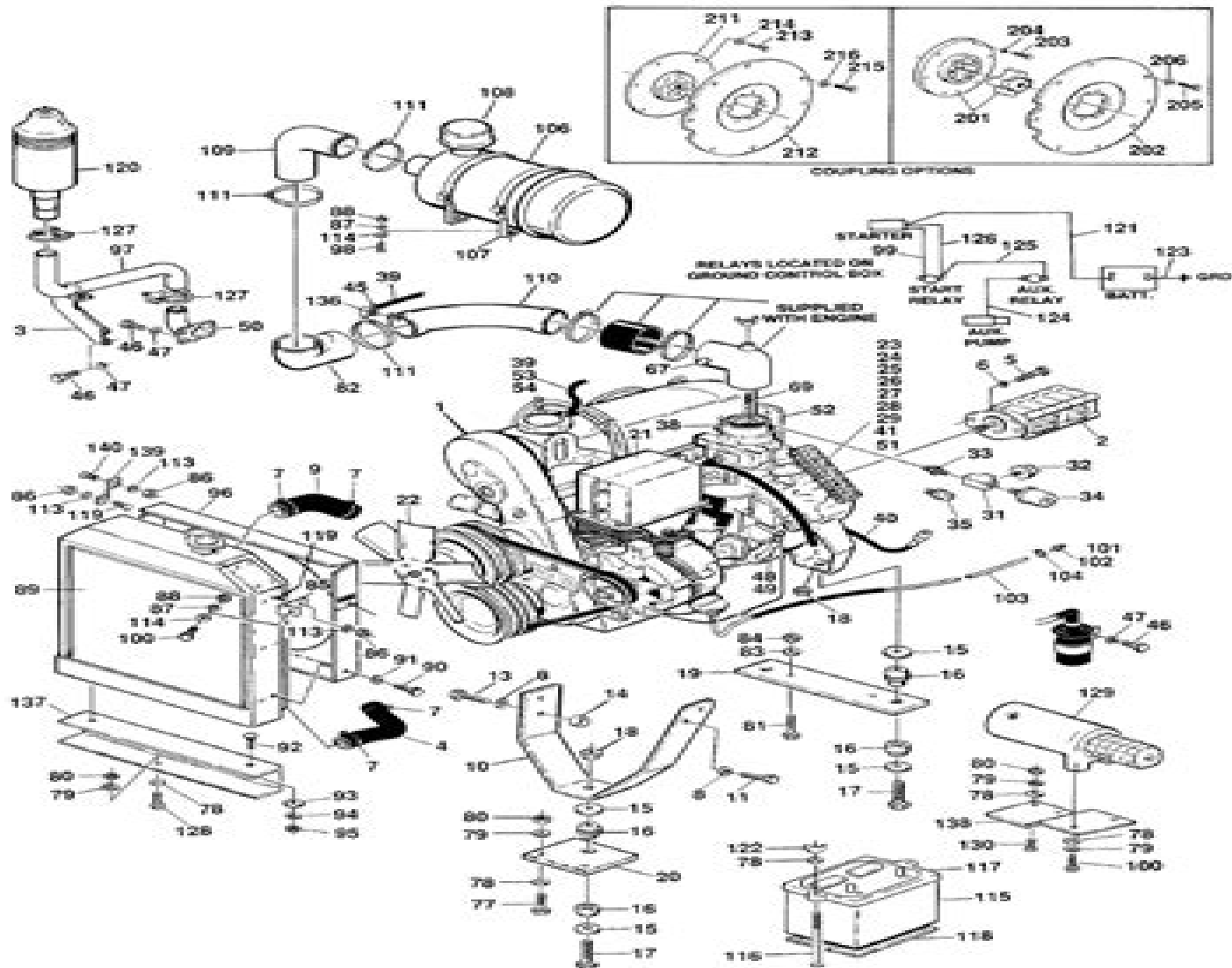
FIGURE 2-17. FORD LSG423 ENGINE INSTALLATION - WITH NOISE REDUCTION (FEBRUARY 1993 TO FEBRUARY 1995)
