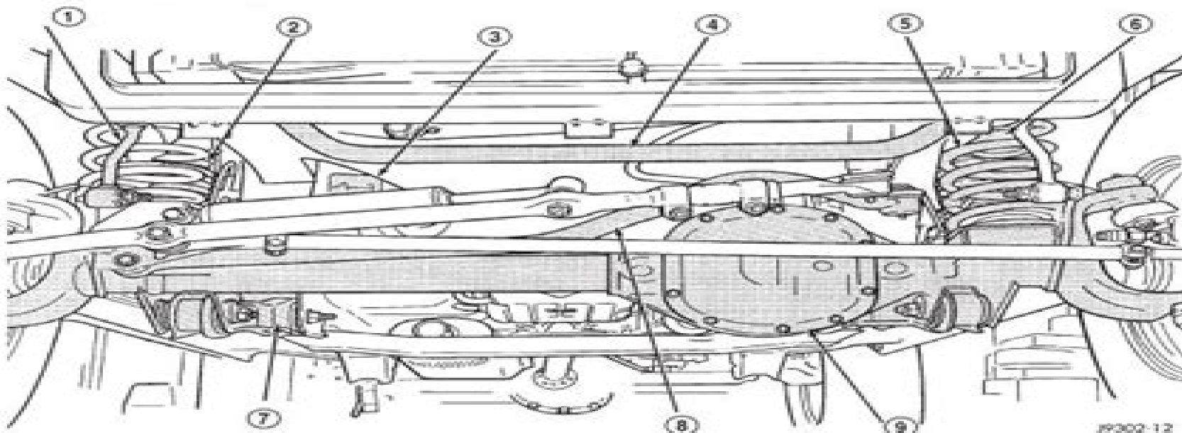
Fig. 1 Suspension Components (LHD)
