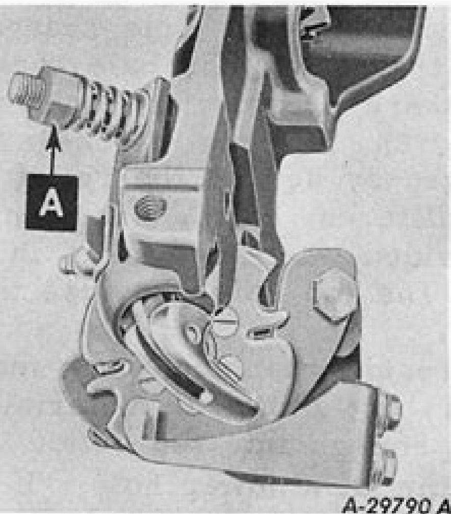
Illust. 20D - Front view of knotter showing tension adjustments.
