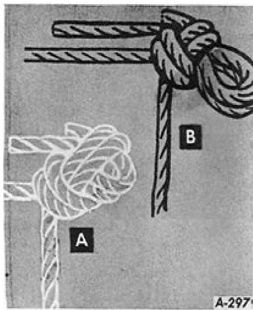
Illust. 20E - Knot "A" is undesirable; knot "B" is correct.
