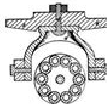
FIG. 5. SECTION THROUGH TRUNNION-PLATE TRUNNIONS AND PIVOT BLOCK.
