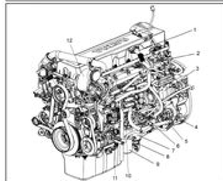
Figure 1. Front view of the Volvo D13 engine (EECU)
