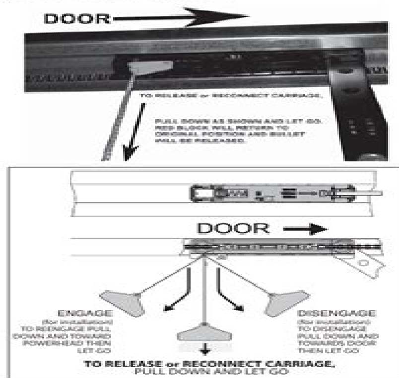
FIG. 6-4 Carriage Release (cut away view)
