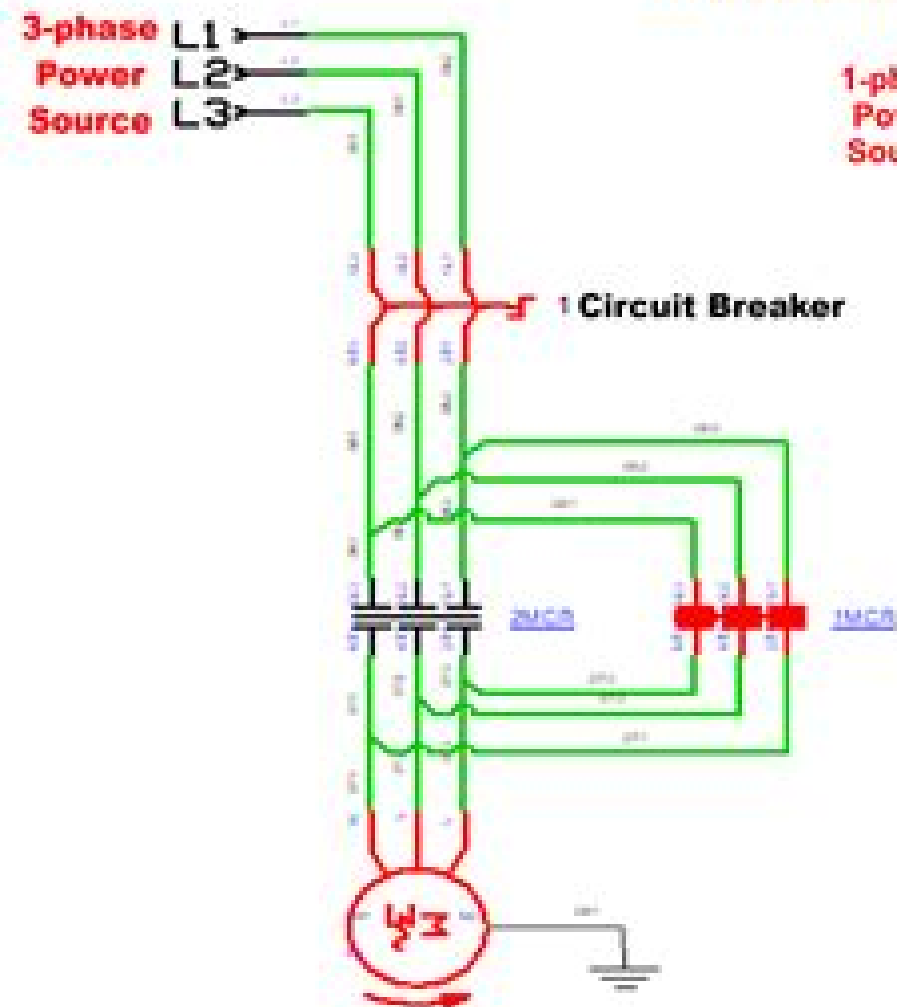
POWER CIRCUIT
