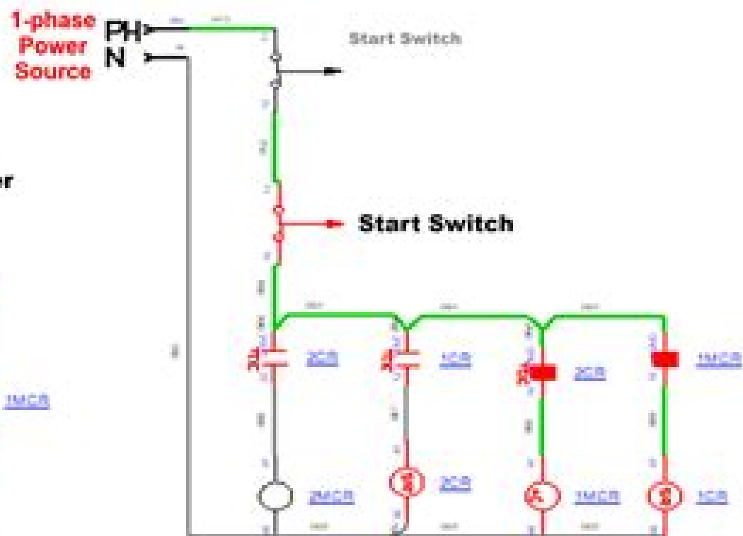
CONTROL CIRCUIT
