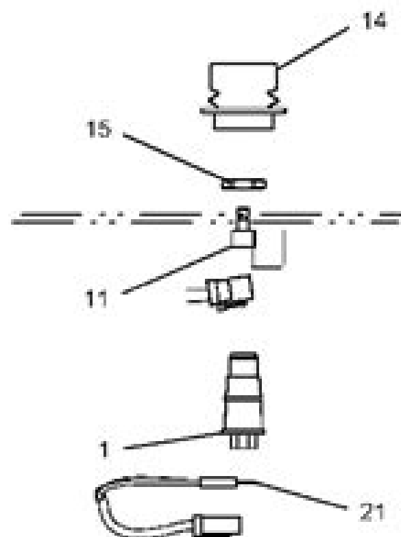
TWO SPEED SWITCH ASSEMBLY
