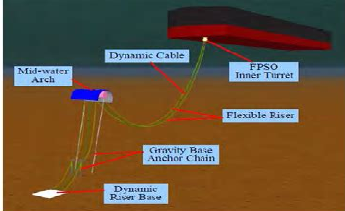
Fig. 1: Dynamic Riser System of FPSO( “Lazy S” Configuration)
