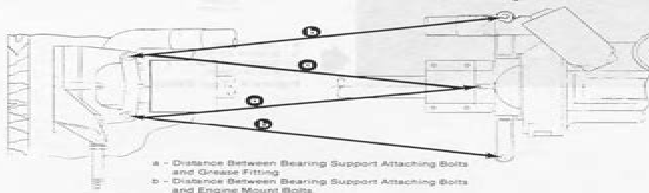
Figure 2. Engine Alignment
