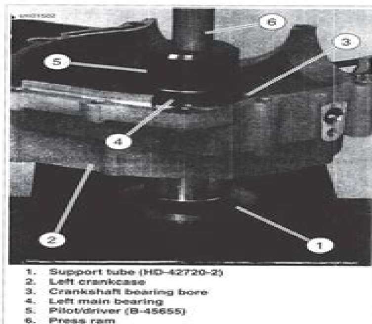
Figure 3-81. Installing Left Main Bearing in Crankcase
