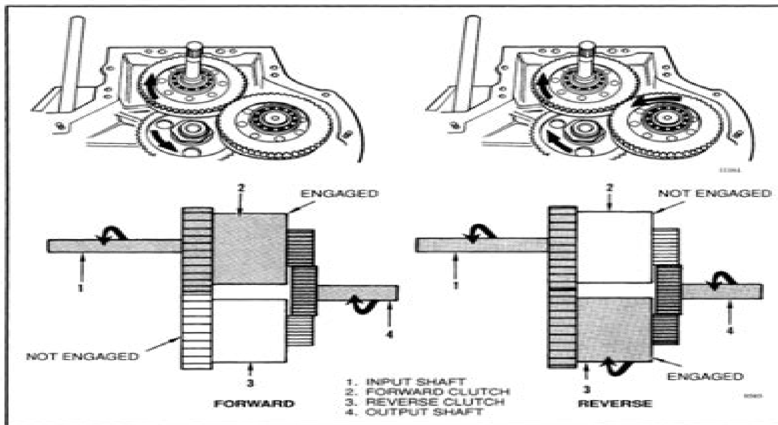
FIGURE 8. CLUTCH OPERATION
