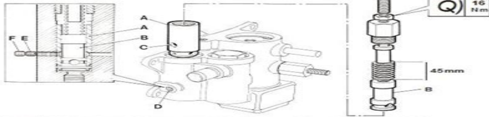
Servo-Valve
