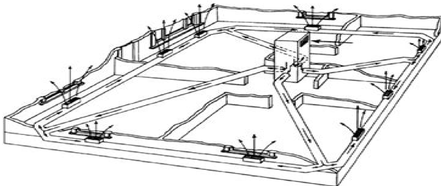
Figure 6-4. Perimeter loop delivery system.
