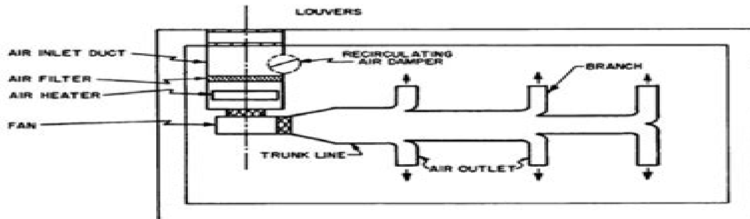
Figure 6-3. Central fan heating system.
