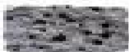
Photomicrograph of andesite.
